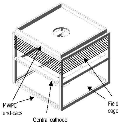
Figure 4: Schematic of the inner part of DRIFT I.
